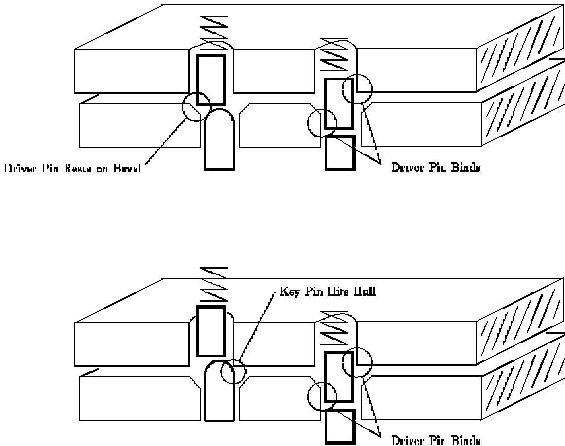
Figure 9.4: Beveled plug holes and rounded key pins
