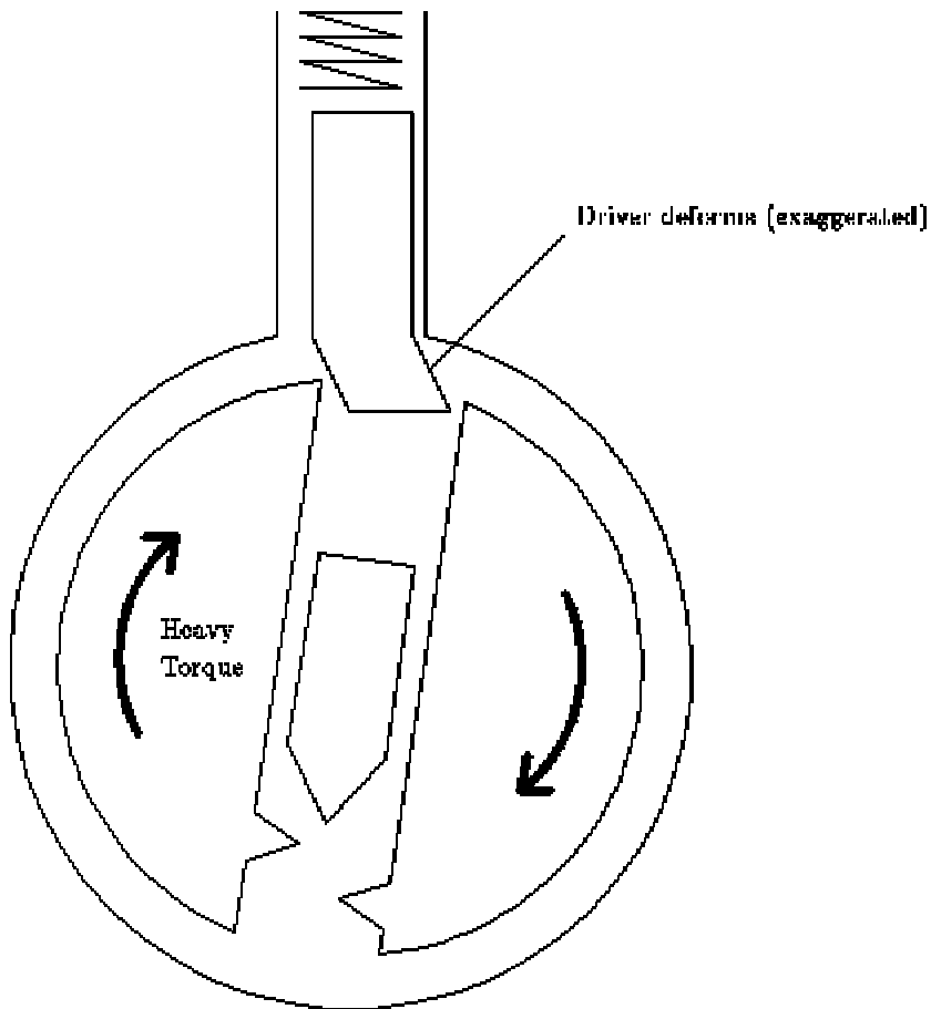
Figure 9.2: Driver pin false set by elastic deformation
