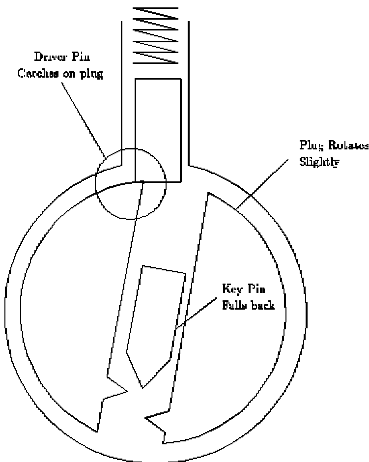
Figure 6.1: Driver pin catches on plug
