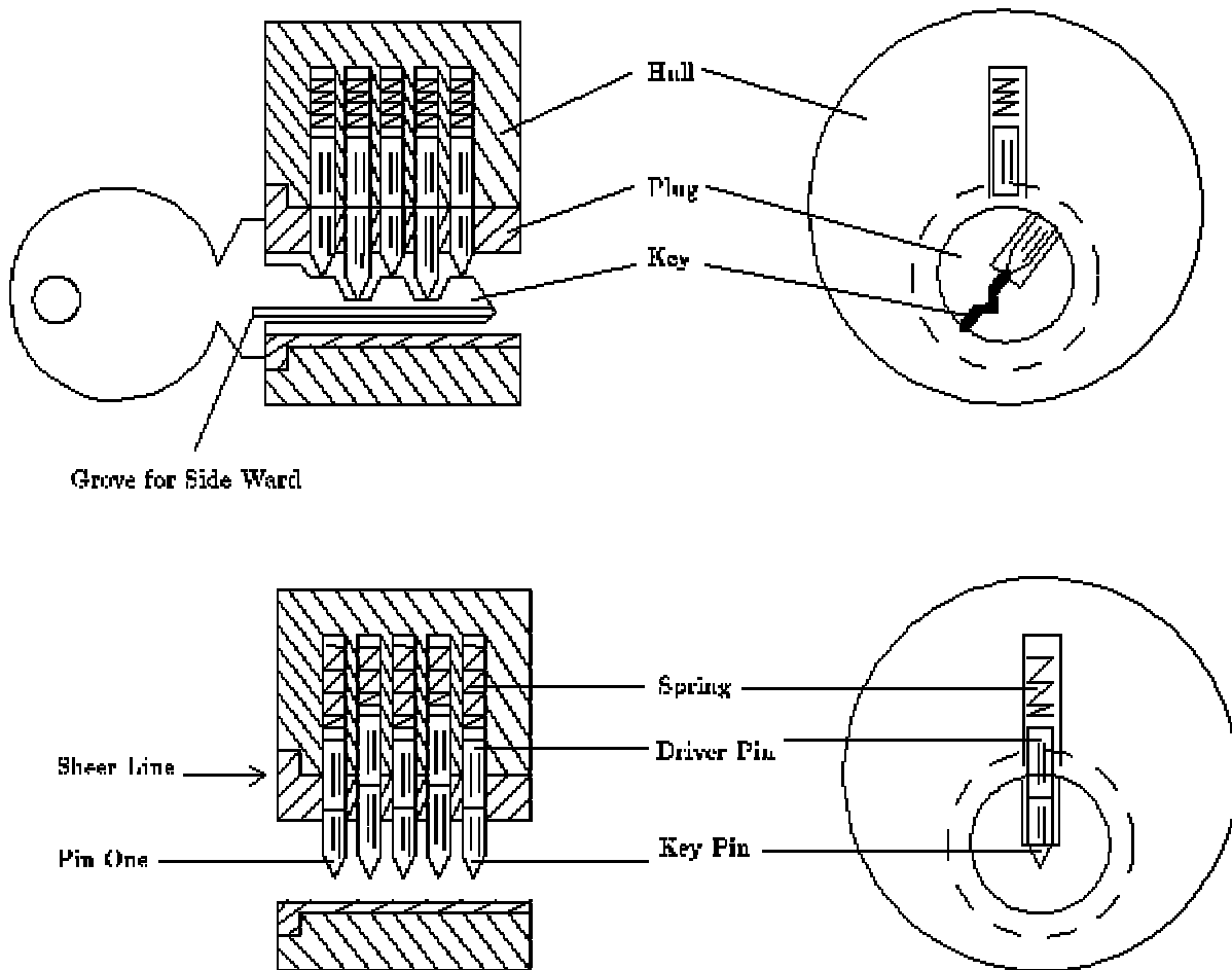
Figure 2.1: Workings of pin tumbler locks
