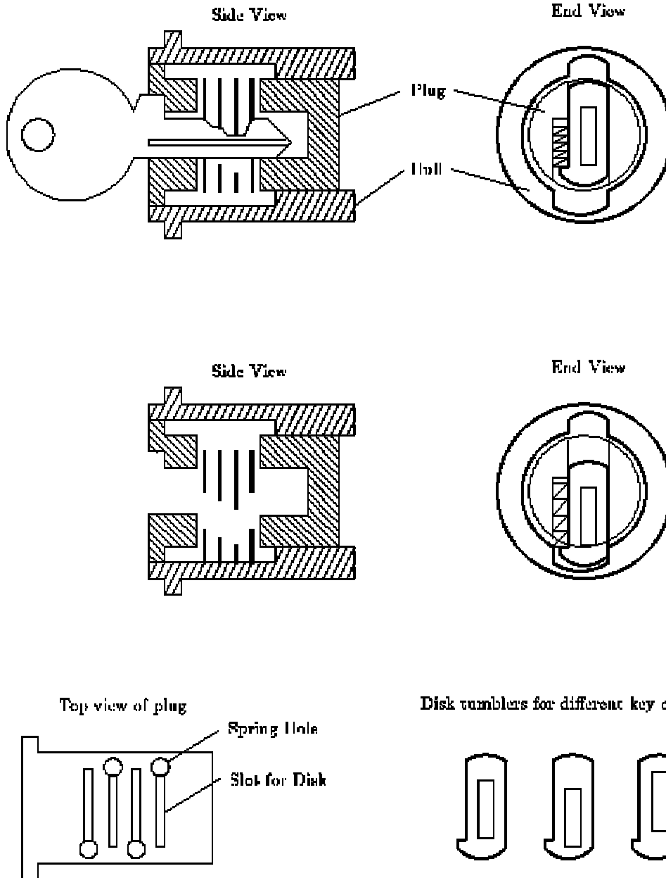
Figure 9.10: Workings of a disk tumbler lock
