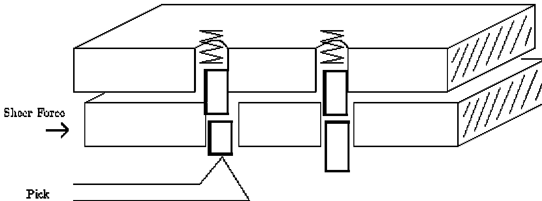
Figure 4.2: (b) Pick lifts the binding pin
