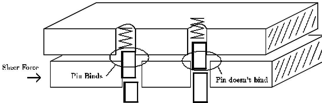
Figure 4.1: (a) Sheer force causes driver to bind
