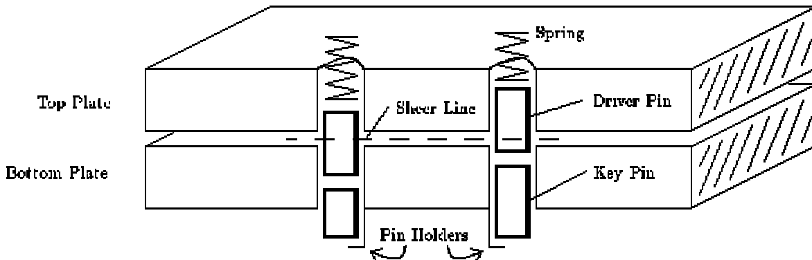
Figure 3.1: Flatland model of a lock
