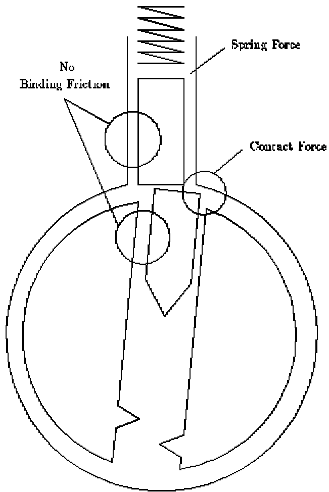
Figure 5.3: Pins at the shear line
