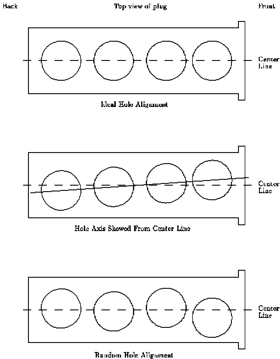
Figure 6.2: Alignment of plugholes
