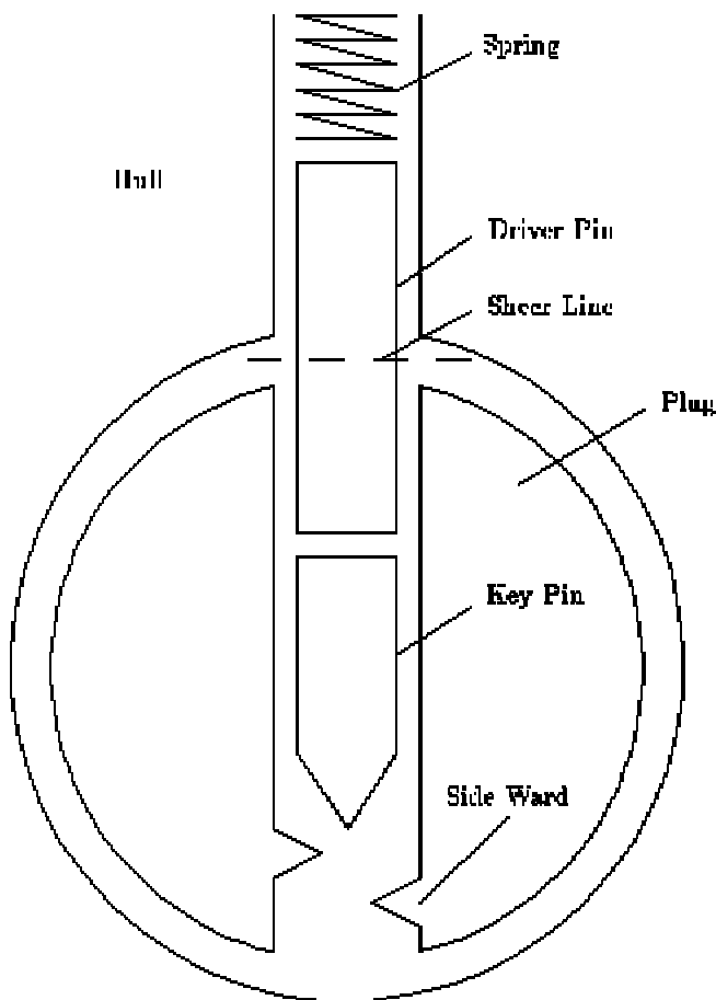
Figure 5.1: The pin-column model
