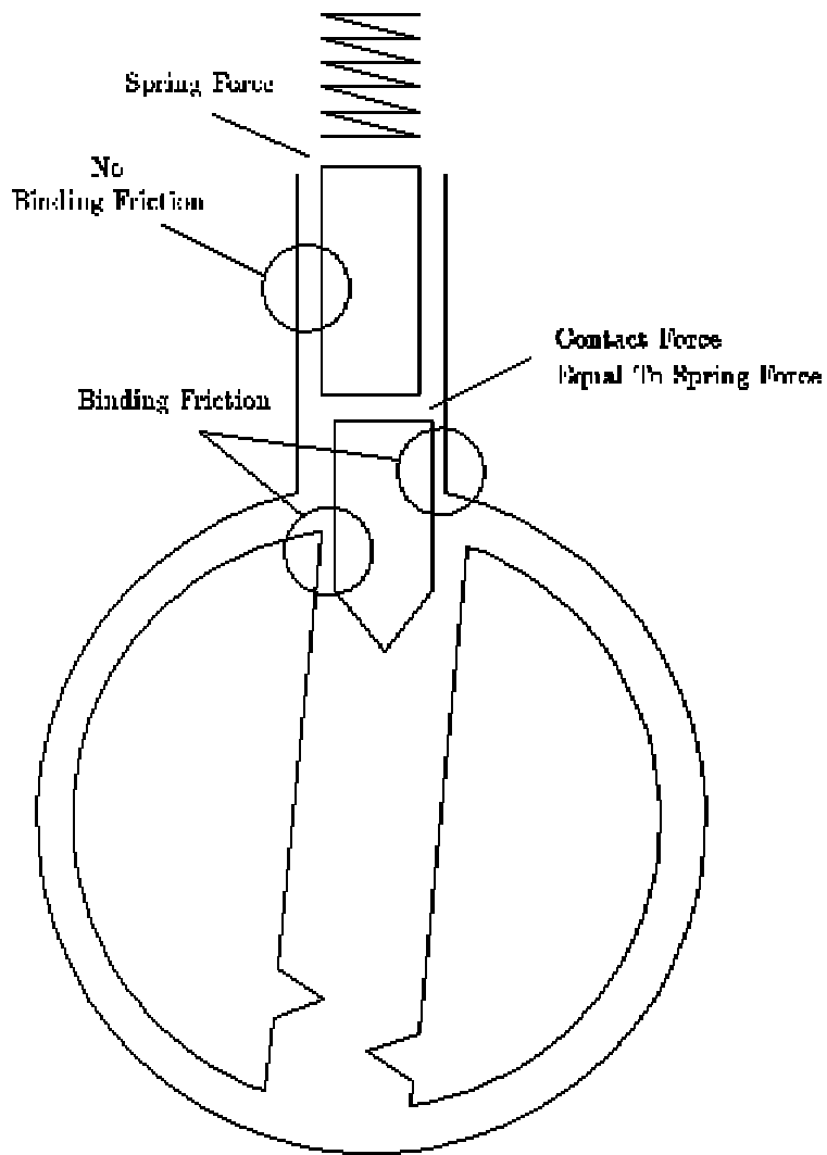
Figure 5.4: Key pin enters hull
