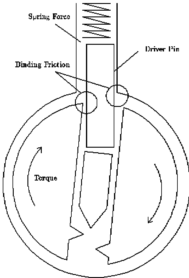
Figure 5.2: Binding in the pin-column model
